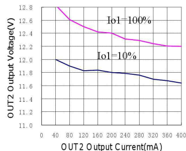
Figure 2: OUT2 Output voltage V.S. OUT2 Output Current
