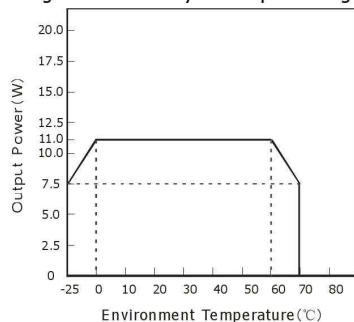
Figure 3: Output Power V.S. Environment Temperature
