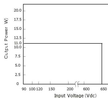
Figure 4: Output Power V.S. Input Voltage
