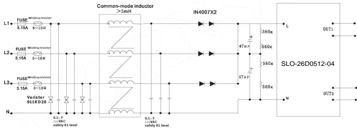
Three-phase-four-wire half-wave rectification application
