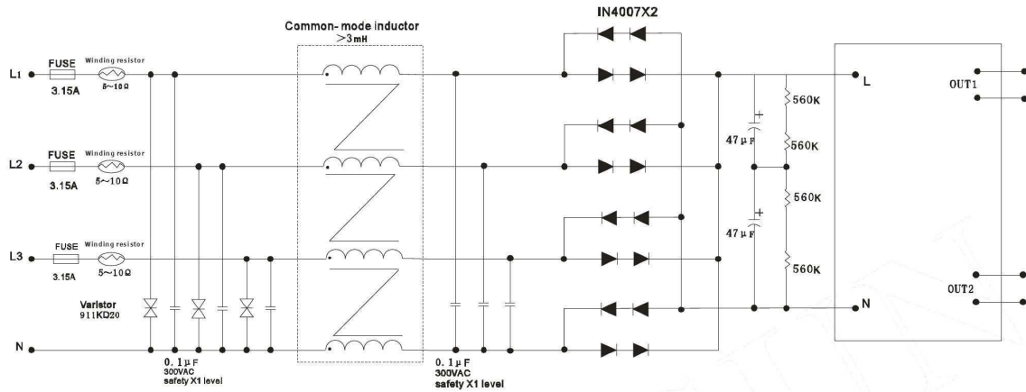
Three-phase-four-wire full-wave rectification application
