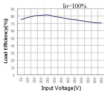
Figure 1: Efficiency V.S. Input Voltage
