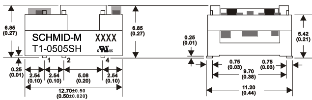
SMD 8Pin Package
