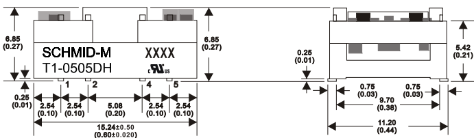
SMD 10Pin Package
