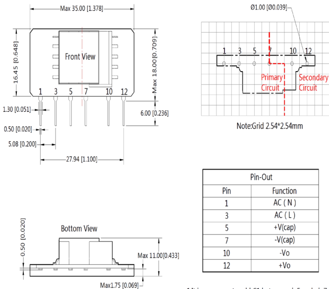
SLS01-15BxxSS Dimensions and Recommended Layout
