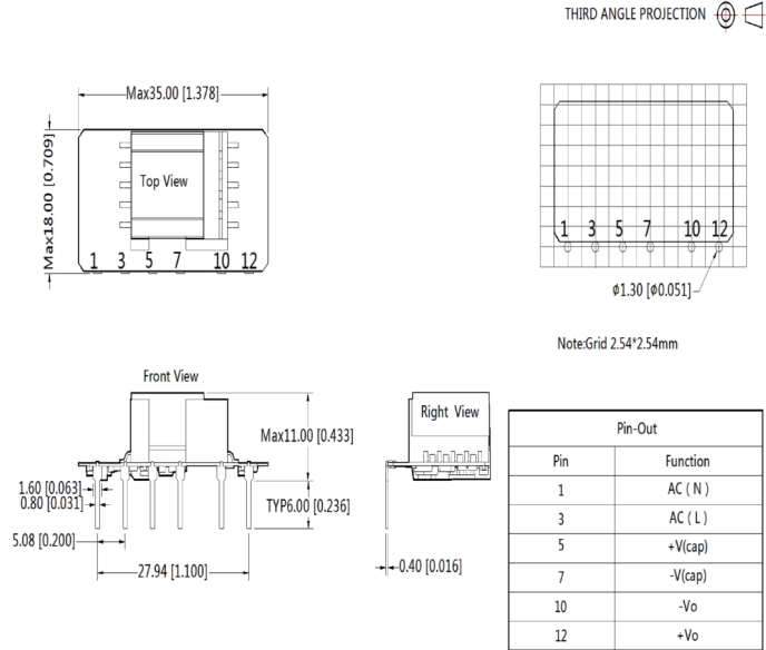
SLS01-15BxxSS-F Dimensions and Recommended Layout
