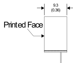
9 Pin SIL Package Non-Conductive Plastic
